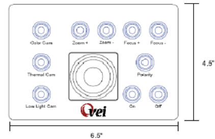
Waterproof Controller
